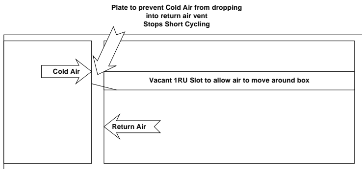
Figure 2 Air Flow allowances inside of case
